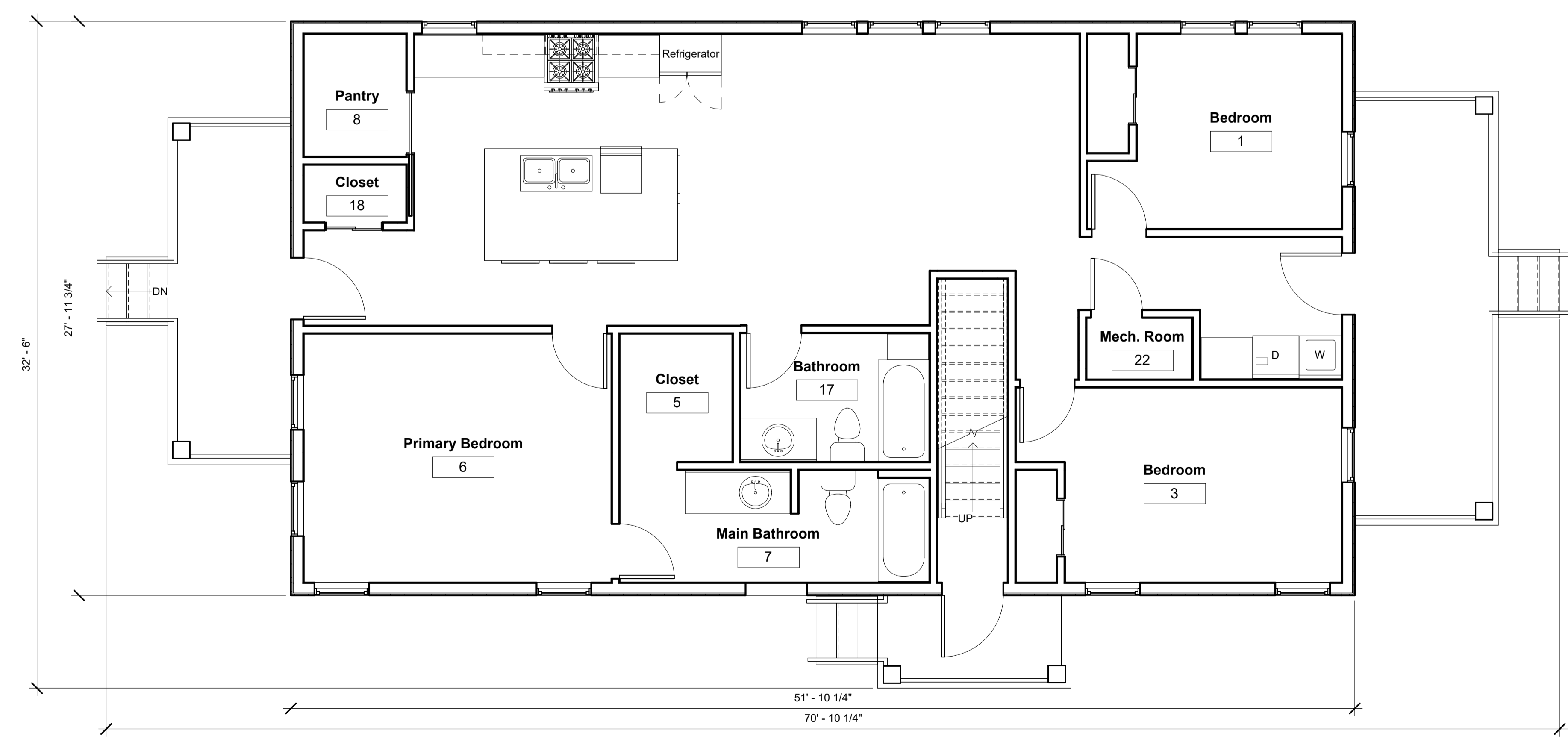
① LEVEL 1 1/4" = 1'-0"
